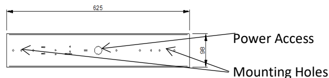
Ceiling Mounting Plate
