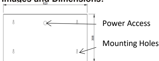
Wall Mounting Plate
